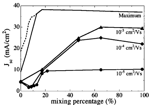
FIG. 2. Short circuit current, J_{sc} , as a function of mixing percentage for different zero-field carrier mobilities. Maximum line assumes all excitons generated are collected, with L_{\text{exc}} = 10 \text{ nm} (all solid lines) and L_{\text{exc}} = 20 \text{ nm} (dashed line).
